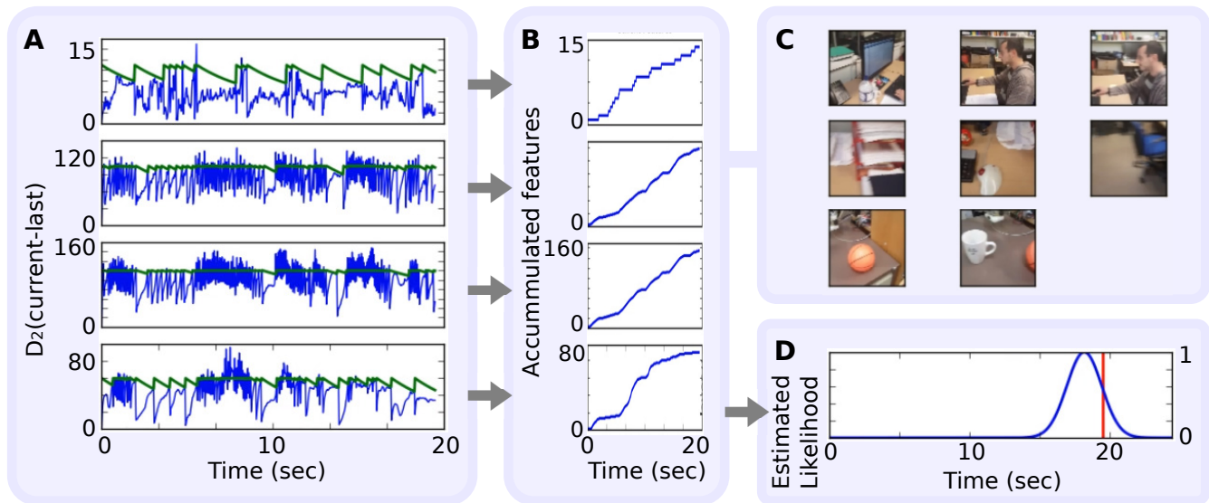
Figure 1: Instance of the time estimation process. A : Distance between the network state in each recorded layer during observation of the current image and the previously-recorded salient frame (blue curves) and the state of the attention threshold (green curves). B : Number of features that have been accumulated in each network layer. C : Frames of the experienced video that were considered salient in the highest network layer. D : Estimated time (blue curve) and ground truth (red line).
