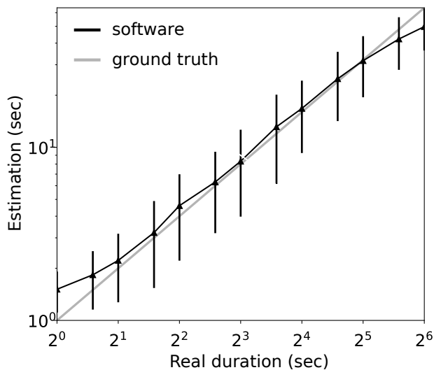
Figure 2: Average performance of the system. The error bars show standard deviation over a sample of 4290 trials.
